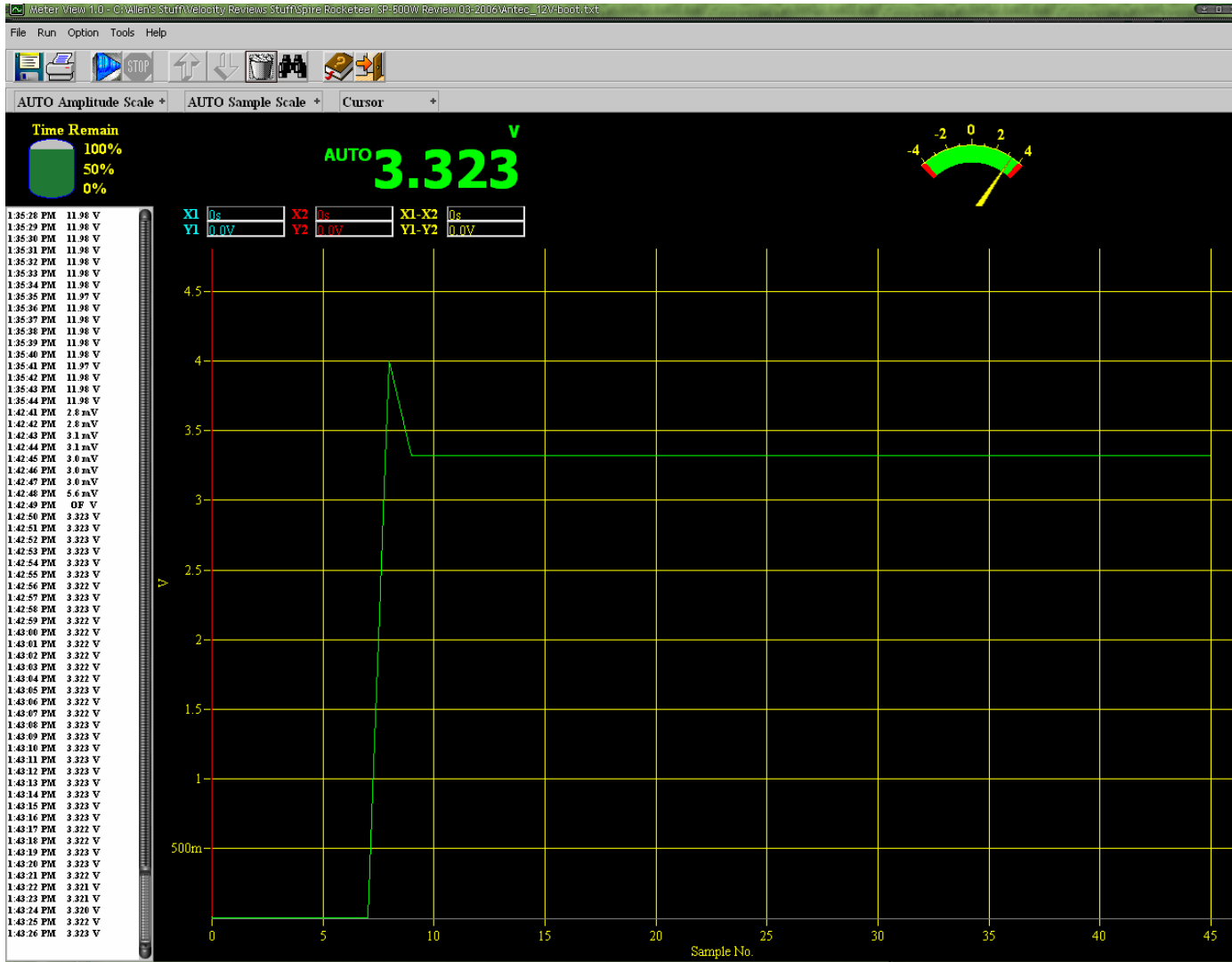
Figure 3 Antec True 480 3.3 Volt boot graph
